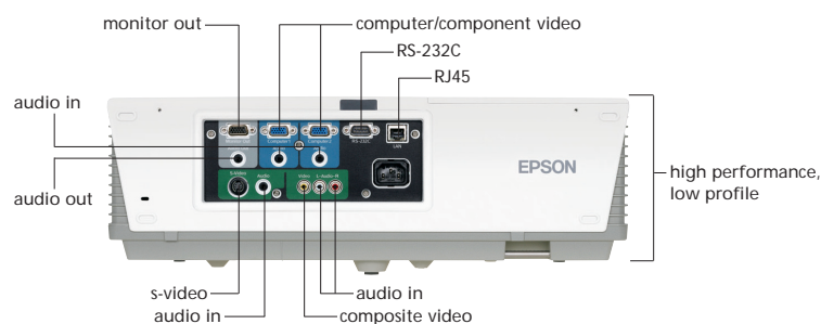
Back View
